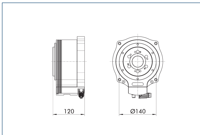
The view shows the height of the ERT with protection class IP54.
