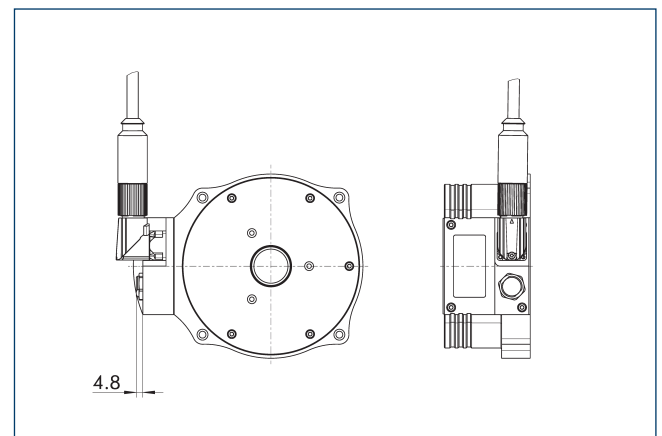
The view shows the ERT with the single-cable technology HIPERFACE DSL®.
