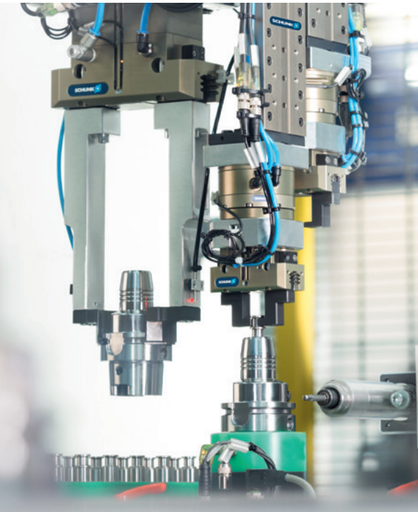
Toolholder balancing
