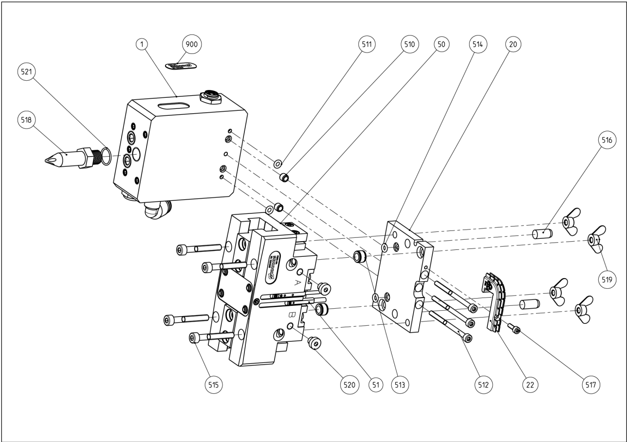
Assembly drawing MTB SG-JGP-P
