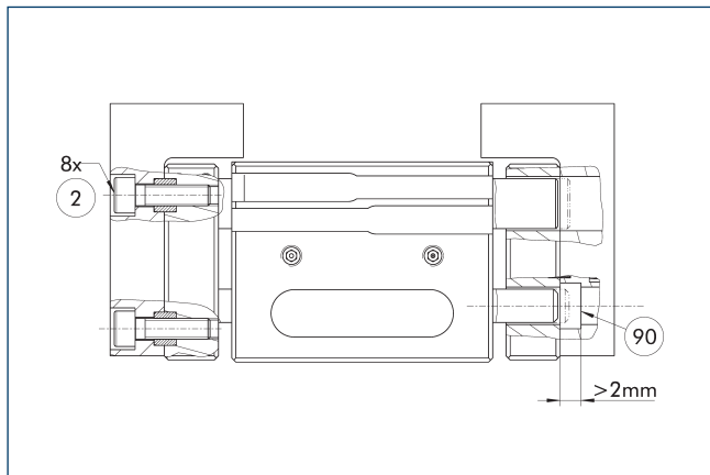
2 Finger connection 90 Recess
