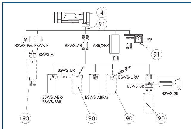
4 Grippers 90 Uniform screw connection pattern 91 Customized gripper fingers
